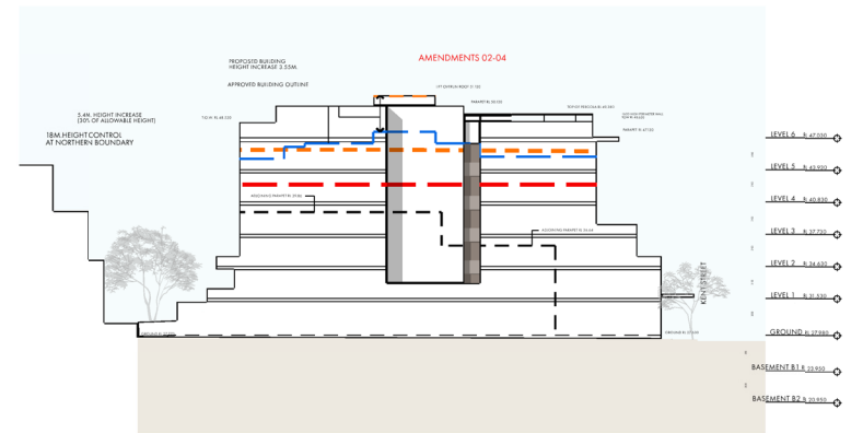
NORTH ELEVATION
